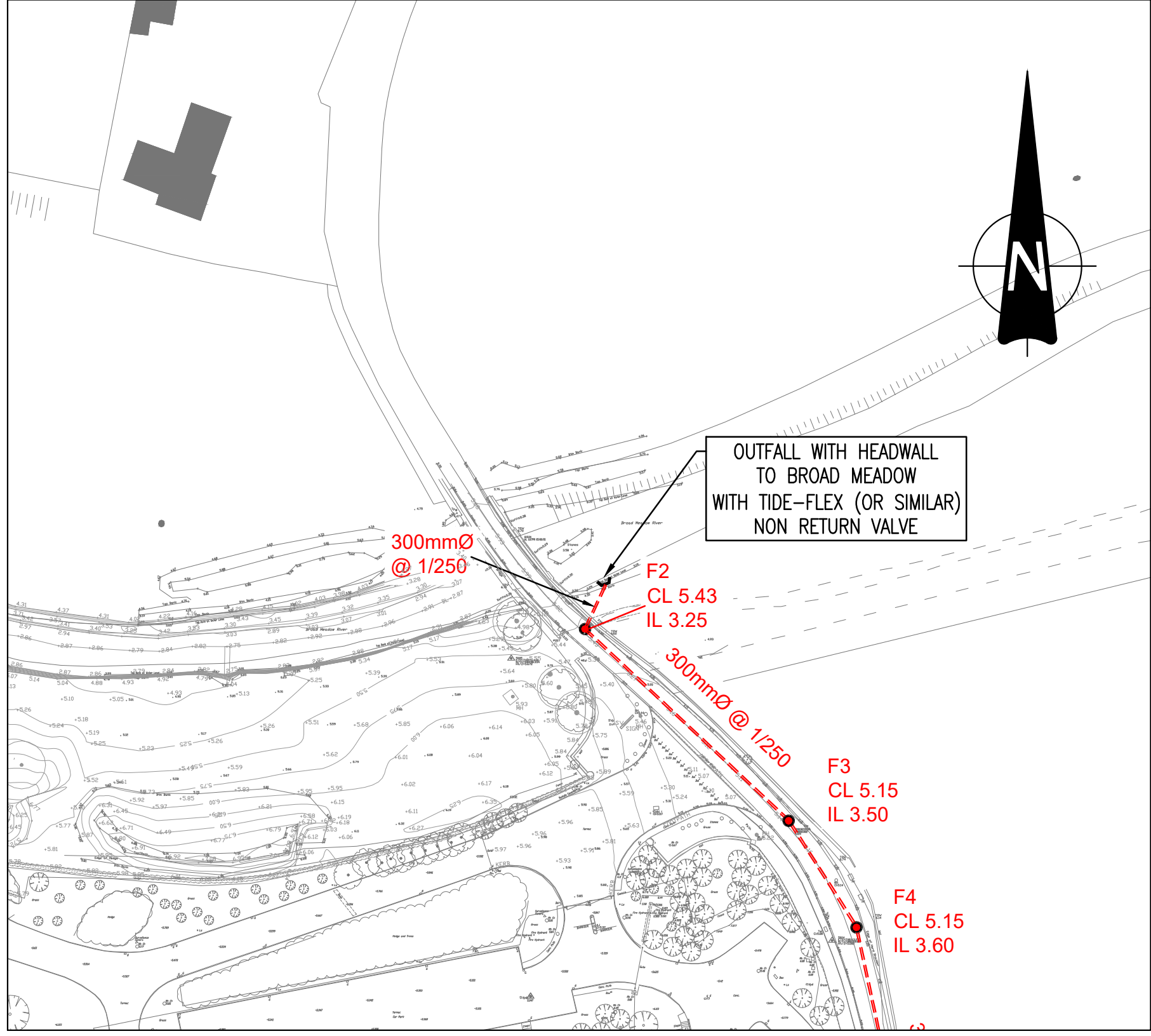
PLAN VIEW – HEADWALL LOCATION SCALE 1:1000 @A1
